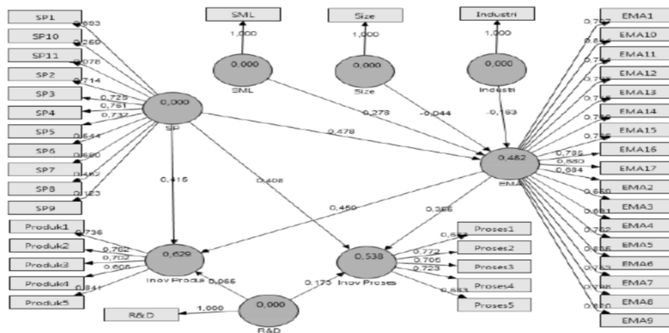
Figure 3: Estimated PLS Path Model Discussion
